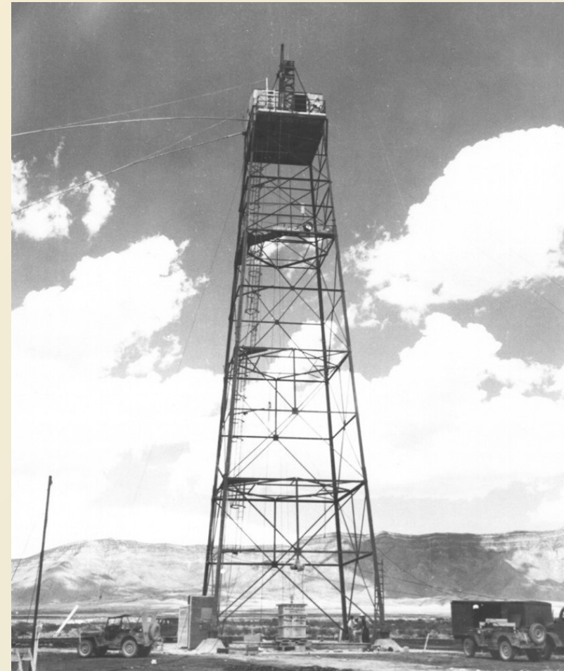
Trinity Test
